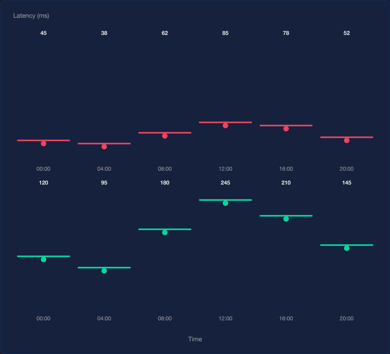
Request Latency (ms)
