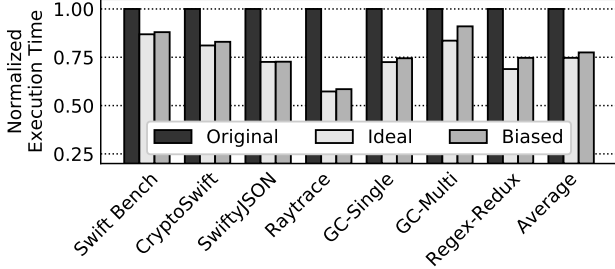
Figure 7: Execution time of client programs under the O , I , and B configurations.
